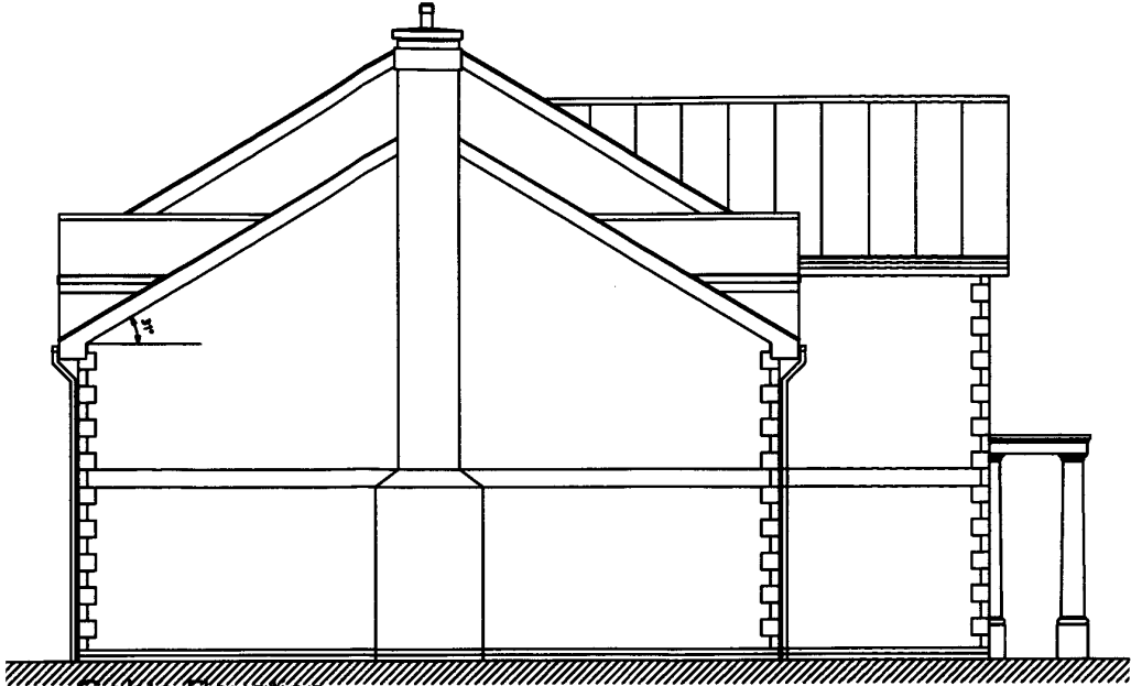
Gable Elevation As Proposed
