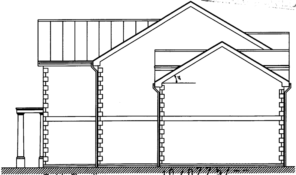
Gable Elevation As Proposed
